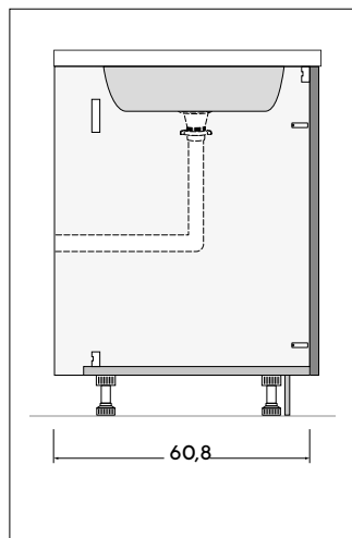
Sezione base lavello H.72 apertura maniglia. H.72 base unit for built-in sink section with handle opening.
